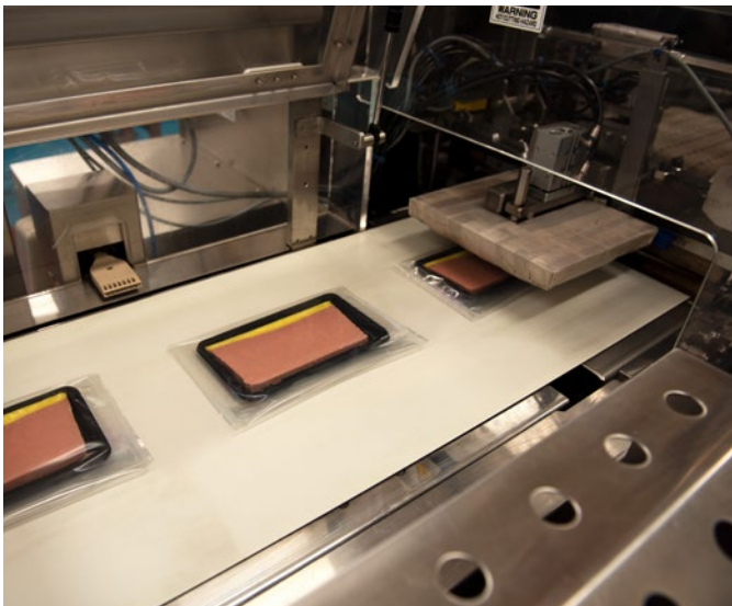
Sensors on the sealing bars detect if there are product, material or folds in the sealing area.
